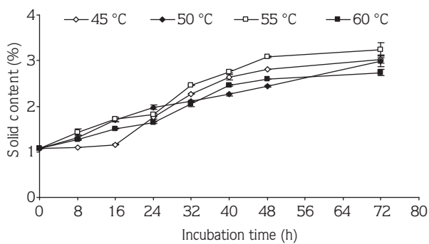
Figure 1. The effect of incubation temperature on total solids content of YE during autolysis.
