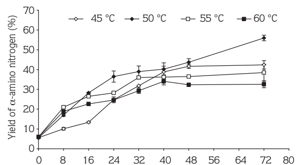
Figure 4. The effect of incubation temperature on \alpha -AN yield of YE during autolysis.
