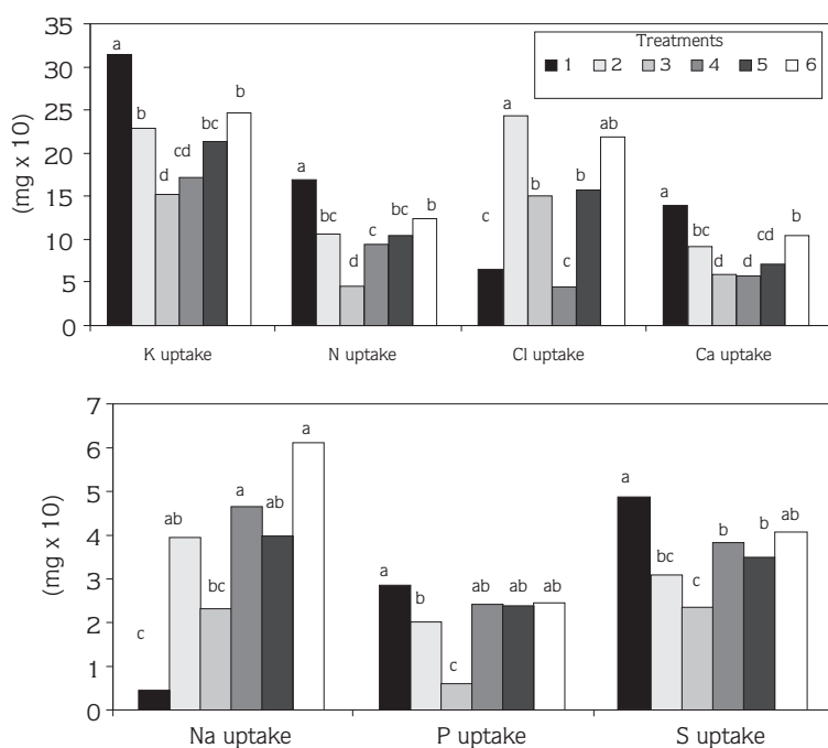
Figure. Uptake rates of K, N, Cl, Ca, Na, P and S ions by tomato plants affected by NaCl and Na 2 SO 4 salinity.
