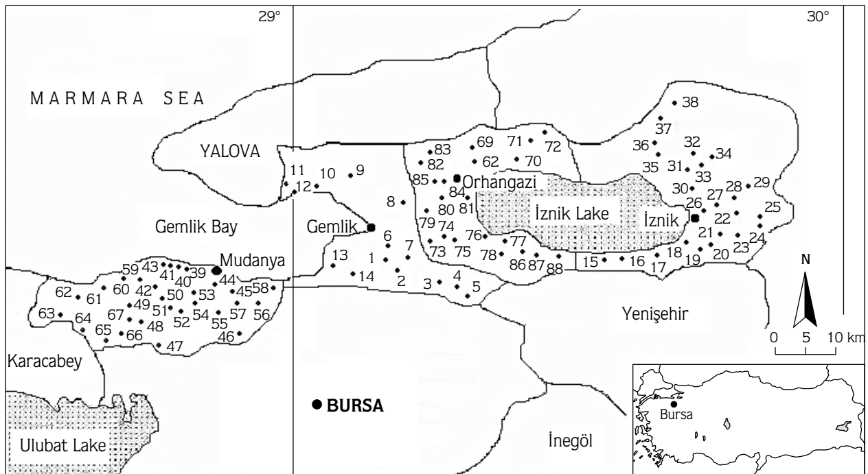
Figure 1. The study area: Localities indicated by numbers (1-88).
