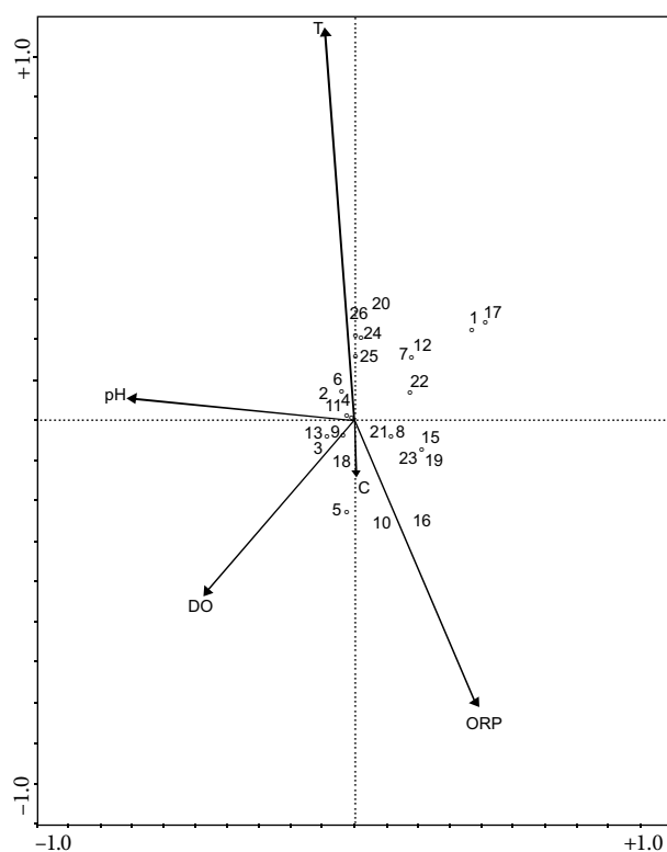
Figure 3. Canonical correspondence analyses (CCA) for depth samples (species scores for taxon names see Table 1).
