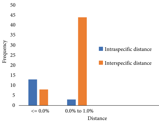
Figure 1. Distribution of interspecific divergence between congeneric species and intraspecific variation.
