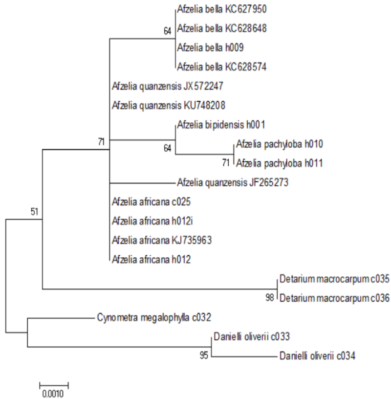
Figure 5. Maximum parsimony phylogram of the original tree; numbers at nodes indicate bootstrap support values.
