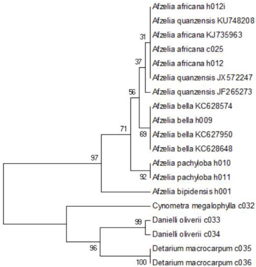
Figure 2. UPGMA cladogram based on K2P model of substitution; numbers at nodes indicate bootstrap support values.
