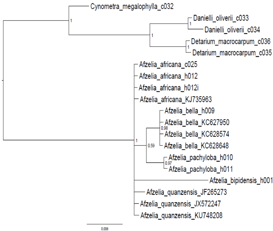
Figure 6. Fifty percent majority consensus phylogram inferred by Bayesian analysis based on GTR model of substitution; numbers at nodes indicate posterior probability value.
