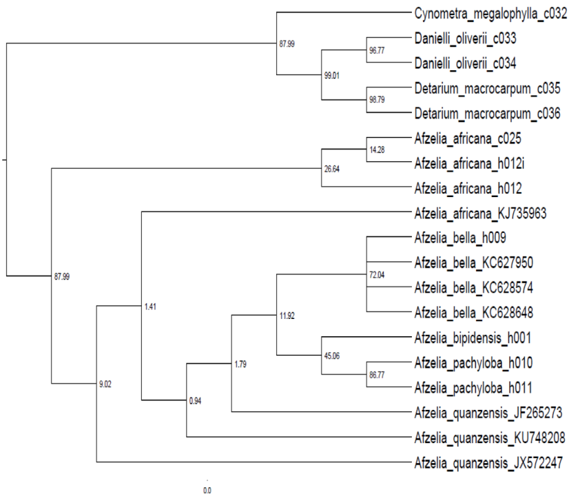
Figure 4. Maximum parsimony phylogram of a strict consensus tree; numbers at nodes indicate bootstrap support values.
