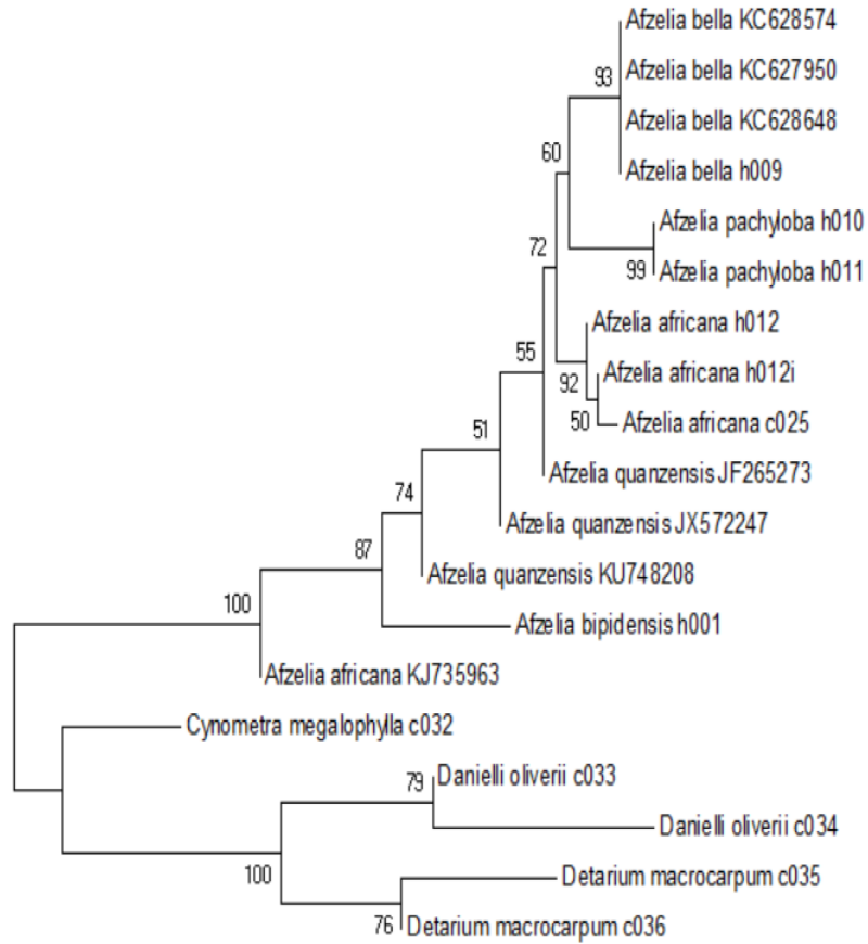
Figure 3. Neighbor joining cladogram based on K2P model of substitution; numbers at nodes indicate bootstrap support values.
