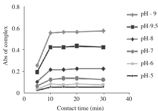
Figure 7. Mefenamic acid-cobalt(II) complex absorbance at various pH values resulting from different contact times, Conditions: 10^{-2} mol/L of drug solution, 50 \mu\text{g/mL} of cobalt(II) solution, agitation rate of 180 rpm and 25^\circ\text{C} .
