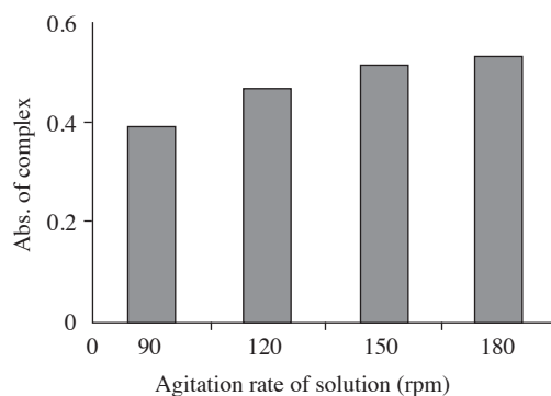
Figure 9. Effect of agitation rate on mefenamic-cobalt(II) complex formation, conditions: pH 9, contact time of 10 min, Initial drug concentration of 10^{-2} mol/L, 50 \mu\text{g}/\text{mL} of cobalt(II) solution and temperature of 25 °C.
