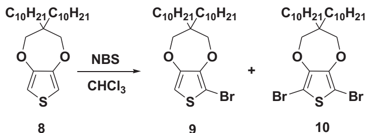
Scheme 2. Bromination of 8.
