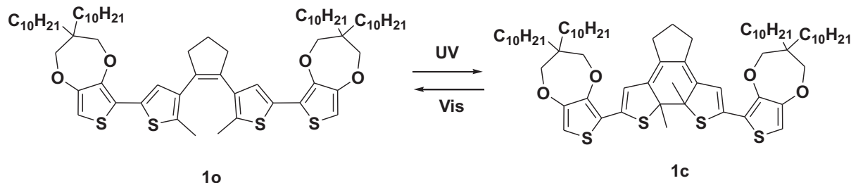
Scheme 4. Photochemical switching of 1o/1c in n -hexane with UV (313 nm) and visible light (>400 nm).
