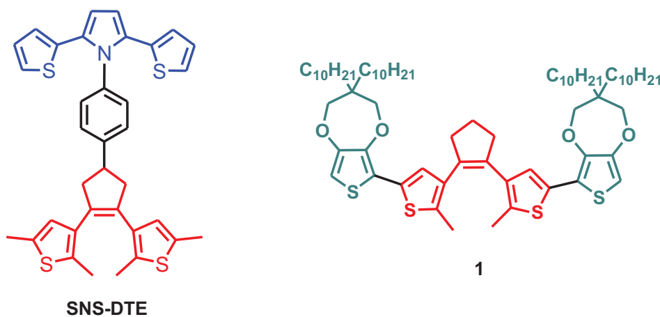
Chart. The structures of SNS-DTE and compound 1 .
