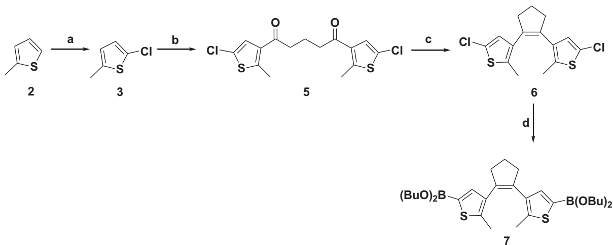
Scheme 1. Synthesis of DTE unit. Reagents: a) NCS, HOAc, \text{C}_6\text{H}_6 , 84%; b) glutaryl dichloride (4), \text{AlCl}_3 , \text{CS}_2 , 83%; c) Zn, \text{TiCl}_3(\text{THF})_3 , THF, 35%; d) n\text{BuLi} , \text{B}(\text{OBu})_3 , THF, 70%.
