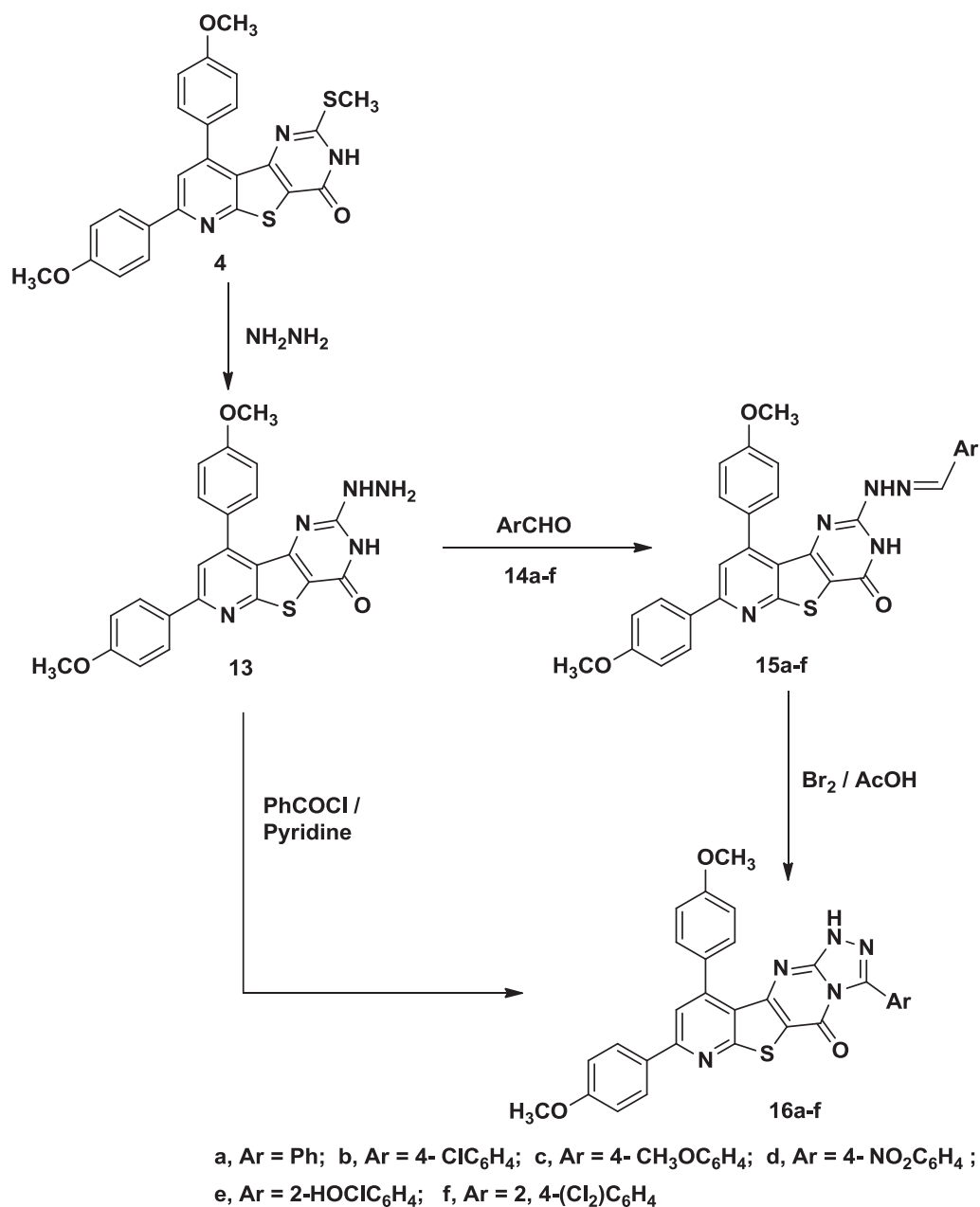
Scheme 4. Synthesis of pyrido[3',2':4,5]thieno[3,2-d][1,2,4]triazolo[4,3-a]pyrimidin-5(1 H )-one ( 16a-f ).
