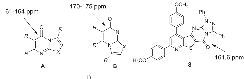
Figure 1. ^{13}\text{C} NMR shifts of strategic carbon atoms.
