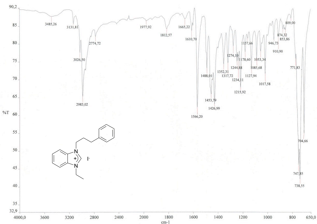
Figure S3. IR spectrum of compound 1b .
