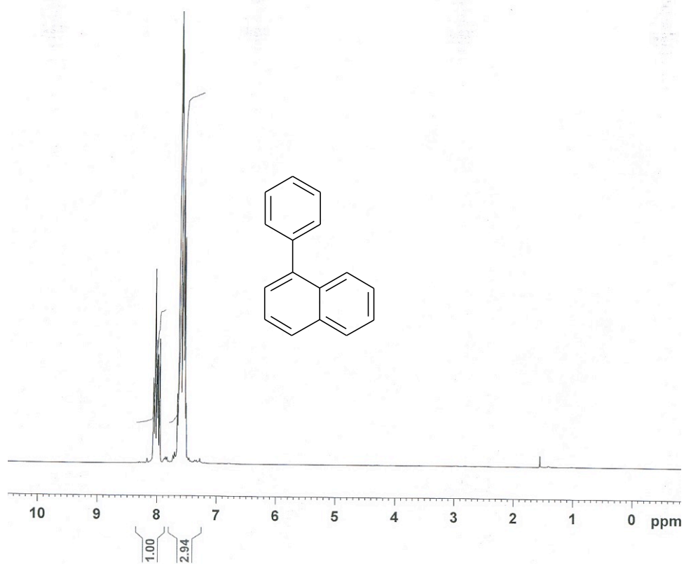
Figure S24. 1 H NMR spectrum of 1-phenylnaphthalene.
