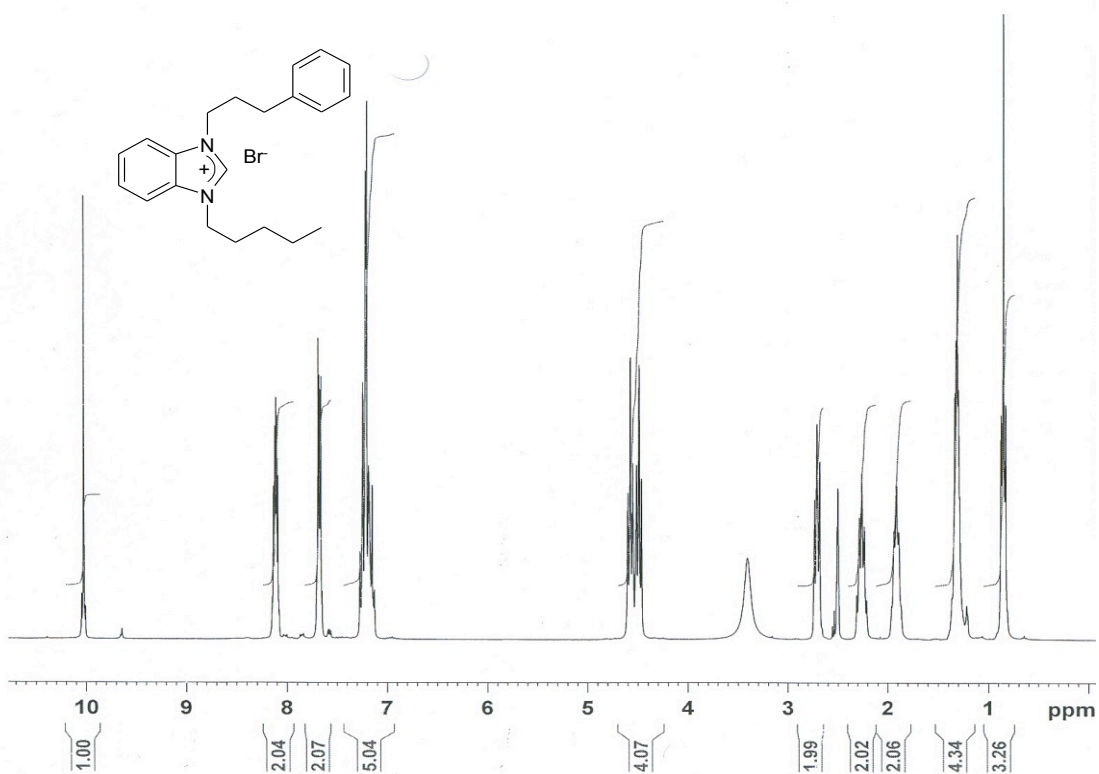
Figure S7. 1 H NMR spectrum of compound 1d.
