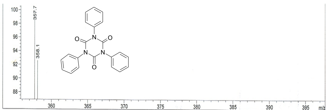
Figure S32. LC-MS chromatogram of 1,3,5-triphenyl-1,3,5-triazinane-2,4,6-trione.
