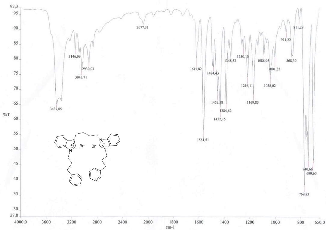
Figure S21. IR spectrum of compound 1h .
