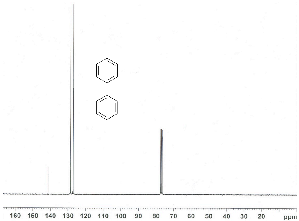
Figure S23. 13 C NMR spectrum of biphenyl.
