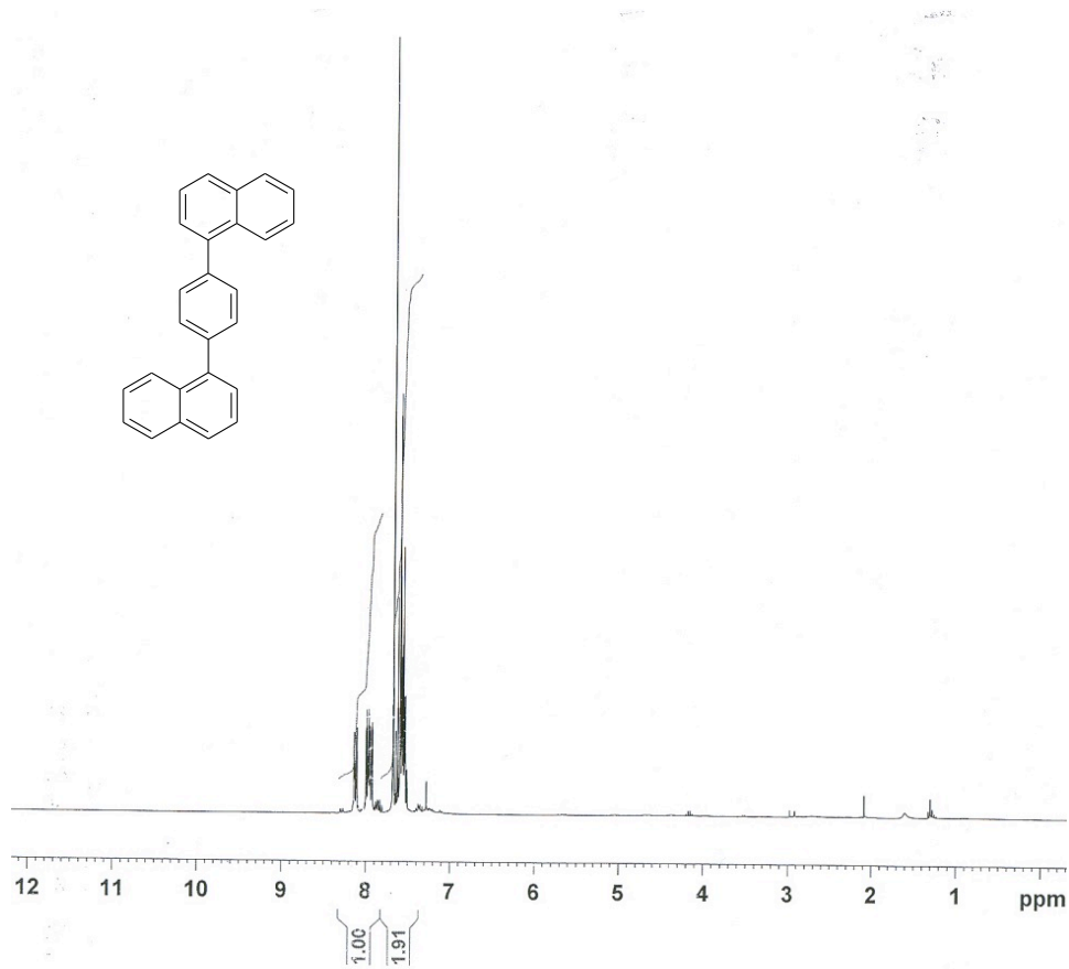
Figure S28. ^1\text{H} NMR spectrum of 1,4-di(naphthalen-1-yl)benzene.
