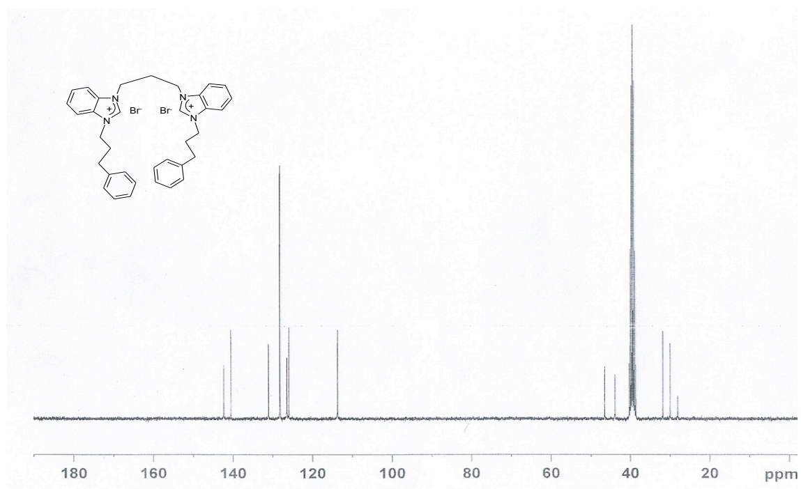
Figure S17. ^{13}\text{C} NMR spectrum of compound 1g .
