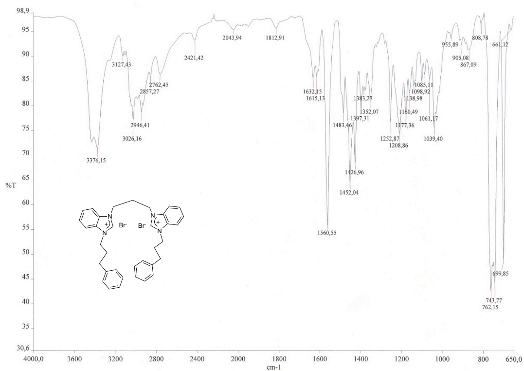
Figure S18. IR spectrum of compound 1g .
