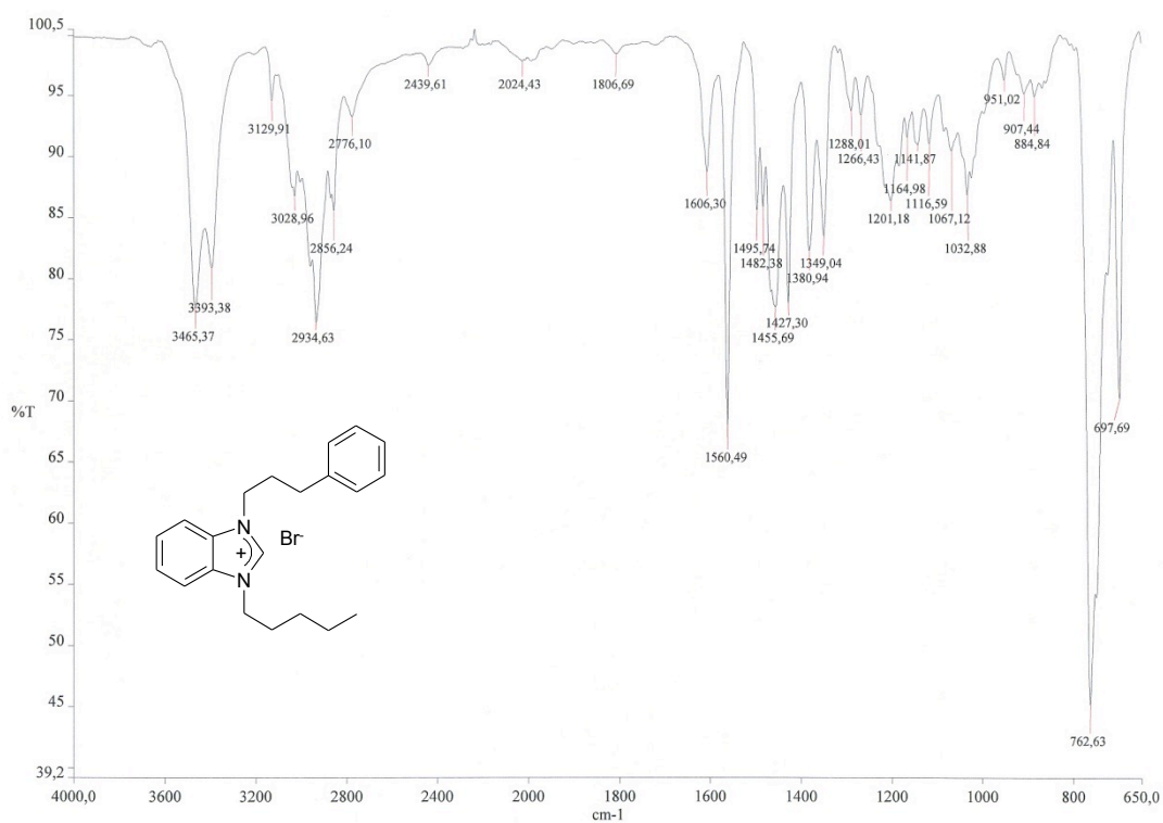
Figure S9. IR spectrum of compound 1d.
