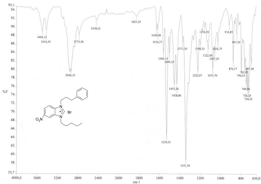
Figure S12. IR spectrum of compound 1e .
