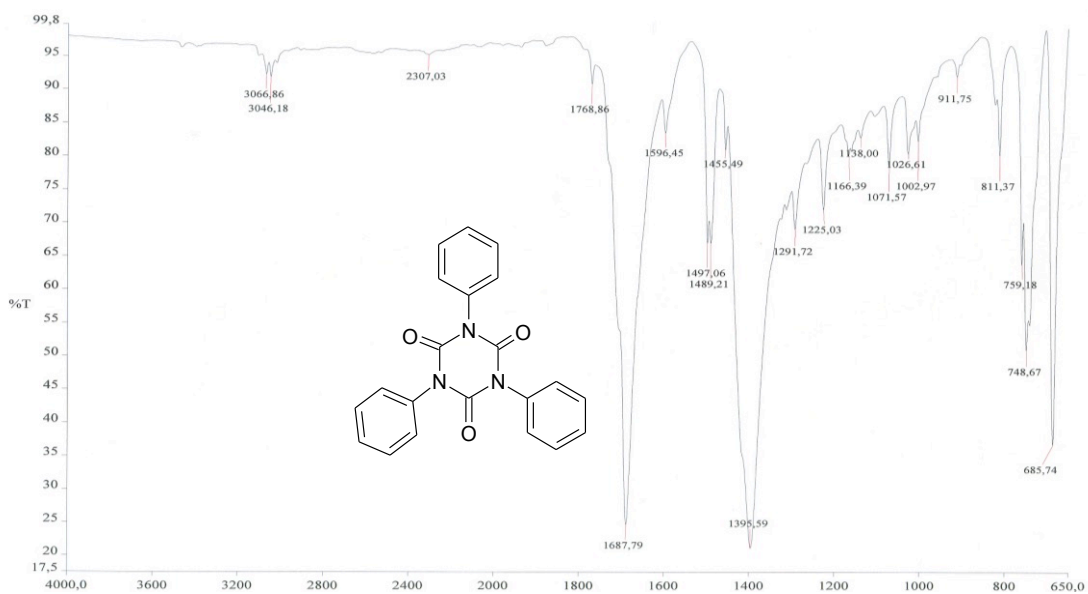
Figure S33. IR spectrum of 1,3,5-triphenyl-1,3,5-triazinane-2,4,6-trione.
