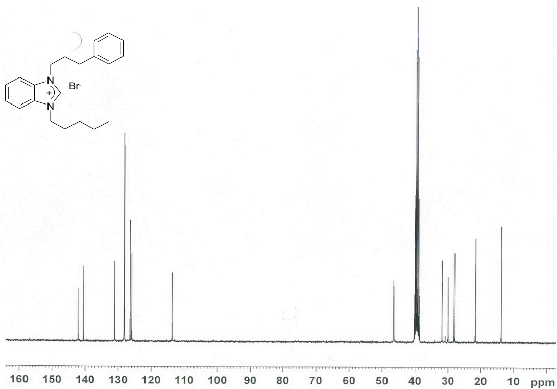
Figure S8. ^{13}\text{C} NMR spectrum of compound 1d.
