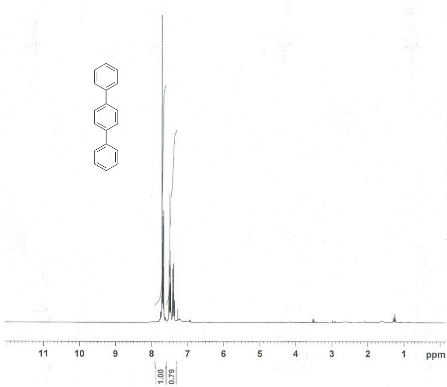
Figure S26. ^1\text{H} NMR spectrum of p -terphenyl.
