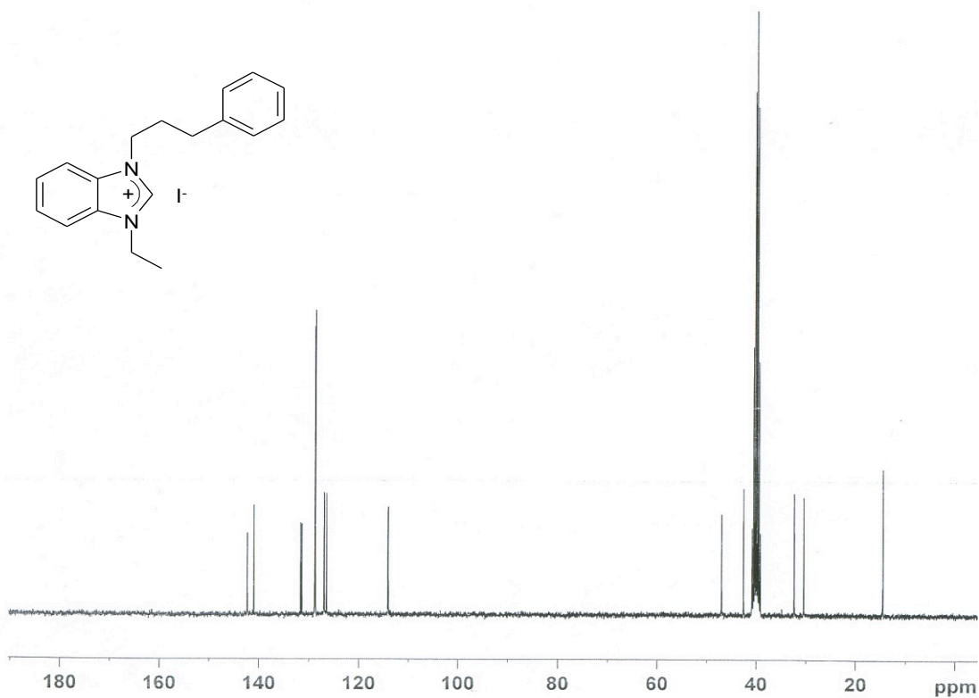
Figure S2. ^{13}\text{C} NMR spectrum of compound 1b .
