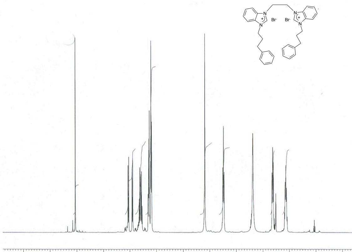
Figure S13. 1 H NMR spectrum of compound 1f .
