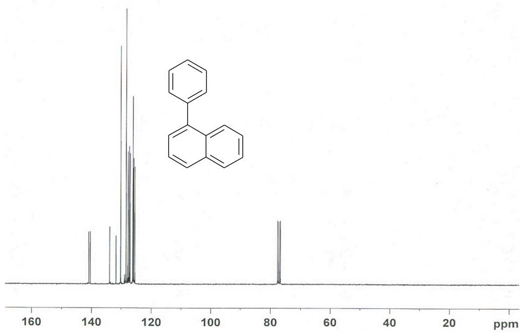
Figure S25. 13 C NMR spectrum of 1-phenylnaphthalene.
