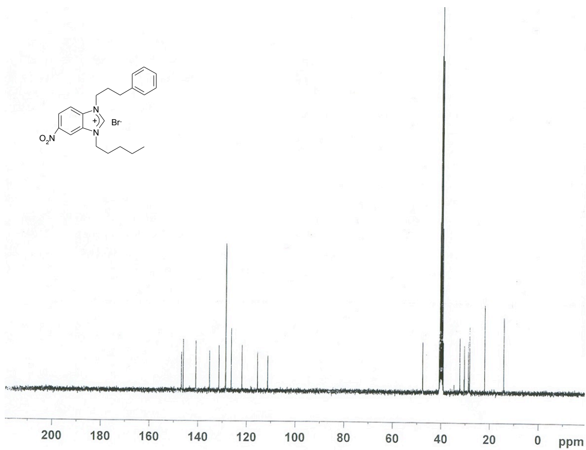
Figure S11. 13 C NMR spectrum of compound 1e.
