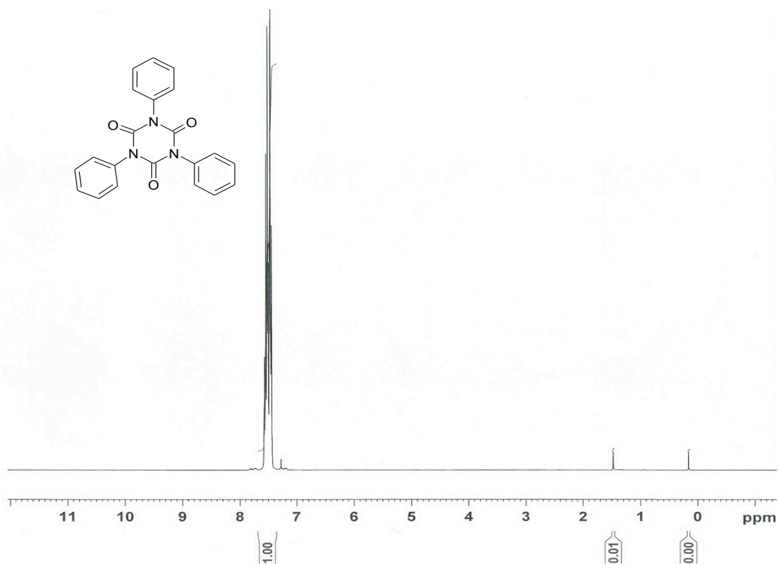
Figure S30. 1 H NMR spectrum of 1,3,5-triphenyl-1,3,5-triazinane-2,4,6-trione.
