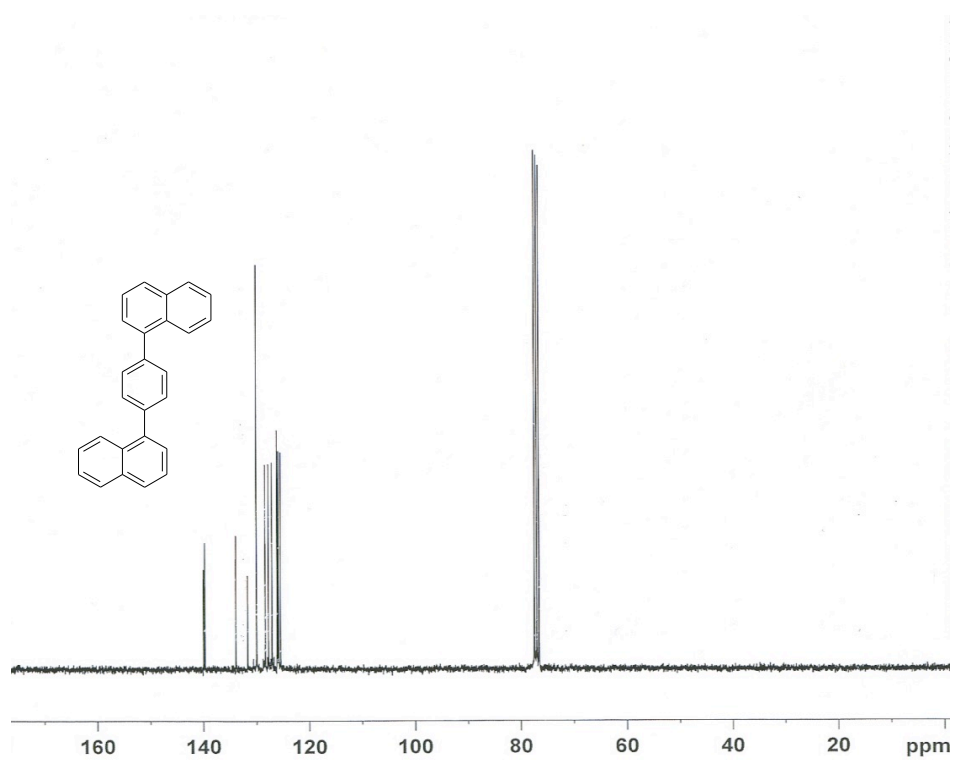
Figure S29. ^{13}\text{C} NMR spectrum of 1,4-di(naphthalen-1-yl)benzene.
