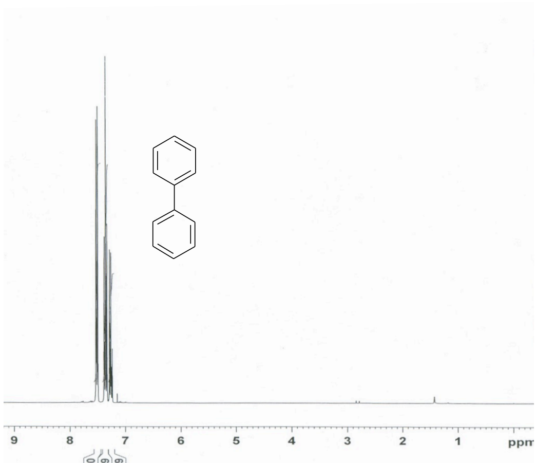
Figure S22. 1 H NMR spectrum of biphenyl.
