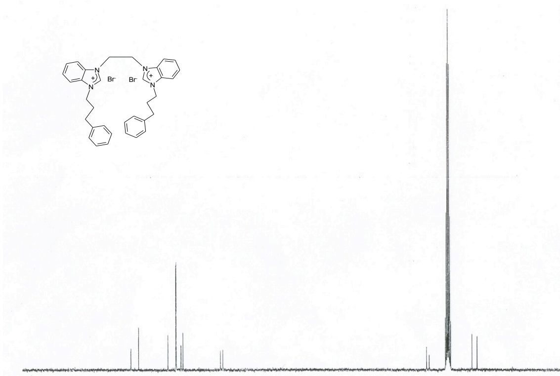
Figure S14. ^{13}\text{C} NMR spectrum of compound 1f .
