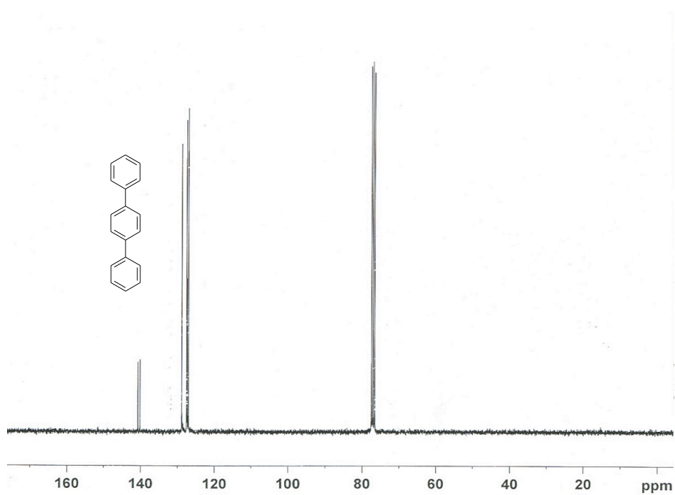
Figure S27. ^{13}\text{C} NMR spectrum of p -terphenyl.
