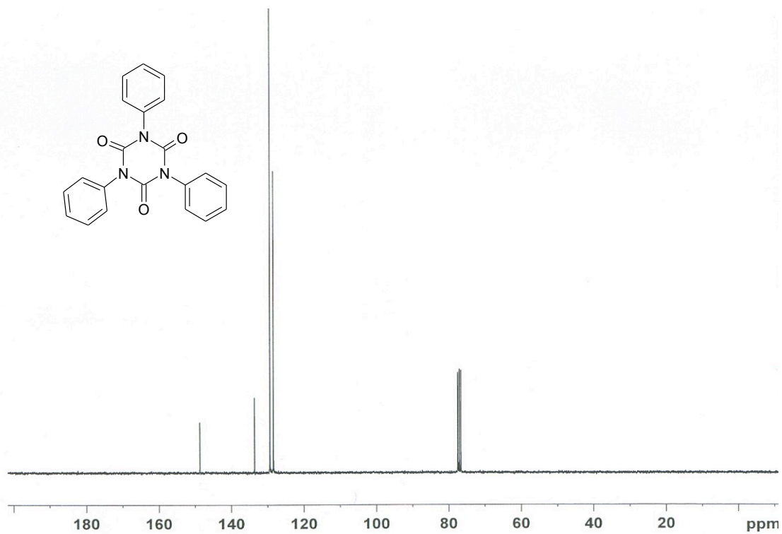
Figure S31. 13 C NMR spectrum of 1,3,5-triphenyl-1,3,5-triazinane-2,4,6-trione.
