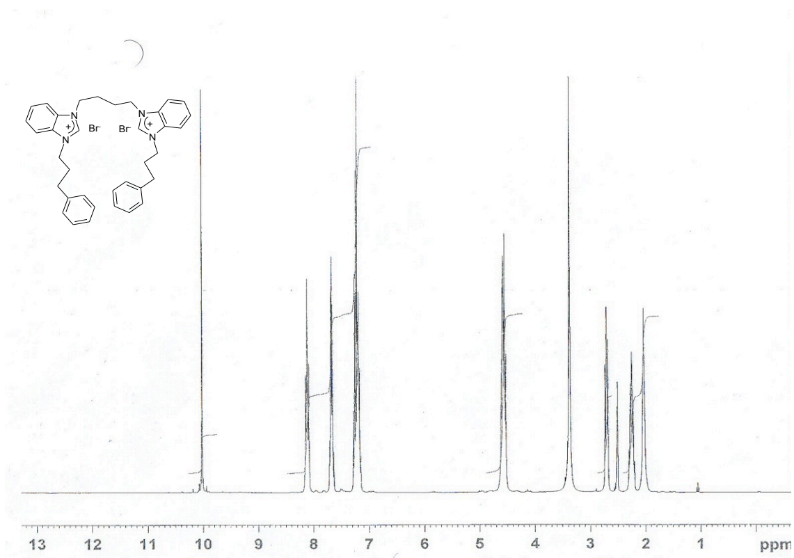
Figure S19. 1 H NMR spectrum of compound 1h .
