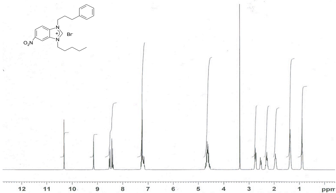
Figure S10. 1 H NMR spectrum of compound 1e.
