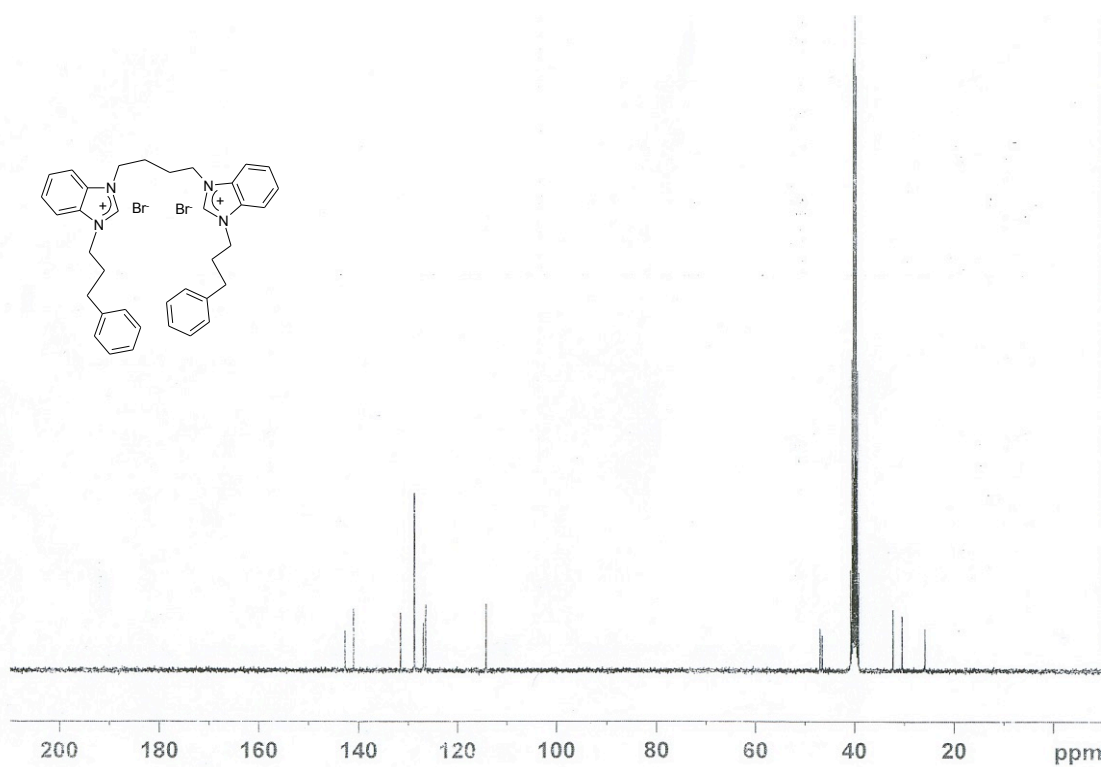
Figure S20. ^{13}\text{C} NMR spectrum of compound 1h .
