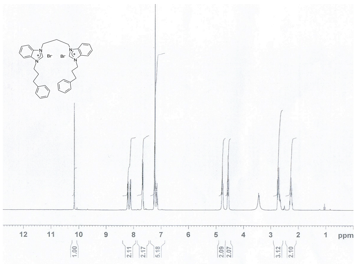
Figure S16. ^1\text{H} NMR spectrum of compound 1g .
