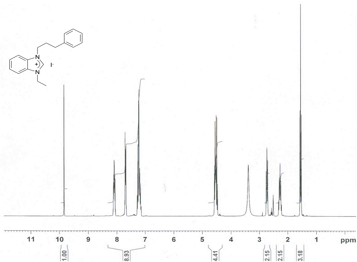
Figure S1. ^1\text{H} NMR spectrum of compound 1b .
