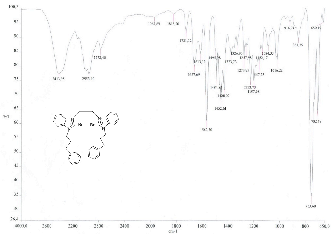
Figure S15. IR spectrum of compound 1f .
