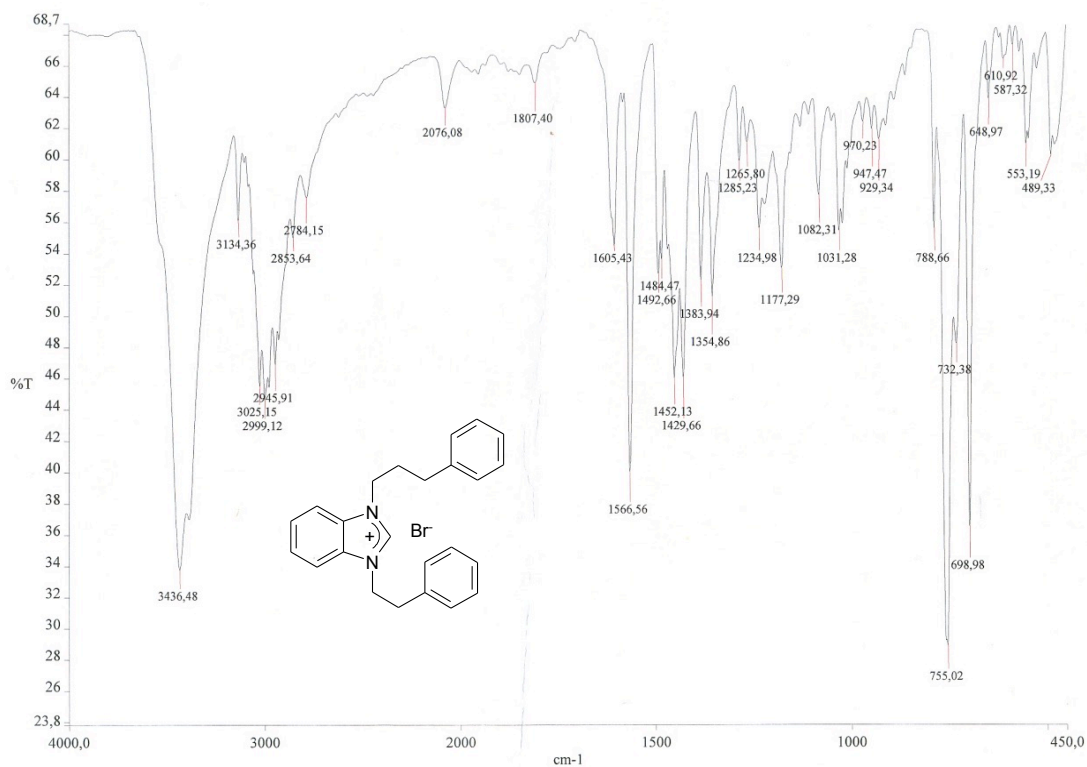
Figure S6. IR spectrum of compound 1c.
