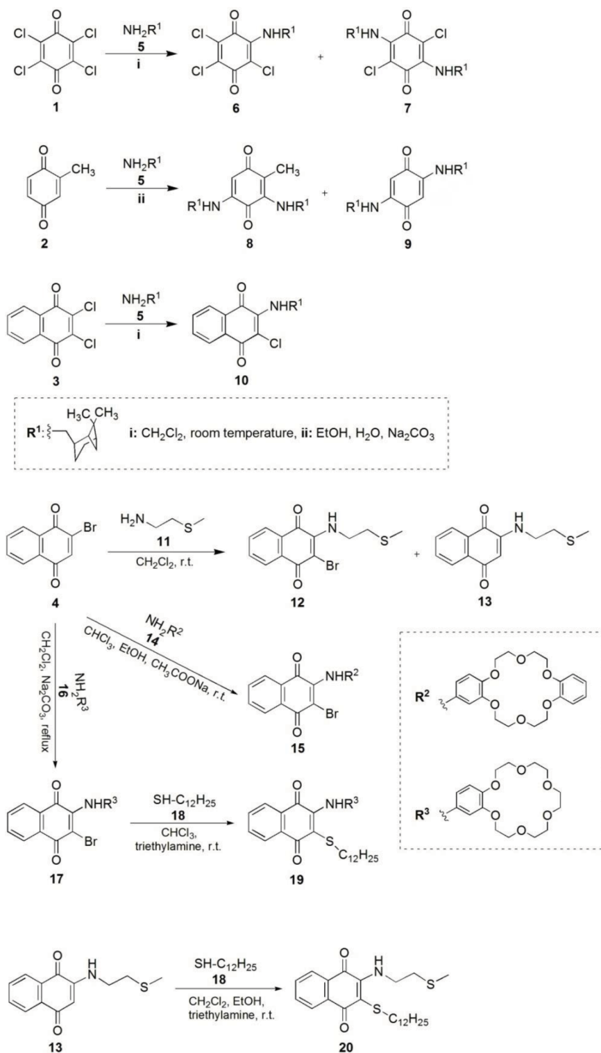
Scheme. The synthesis of compounds 6-10, 12, 13, 15, 17, 19, and 20.
