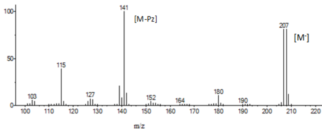
Figure S15. Mass spectrum of NapMe-Pz ligand.
