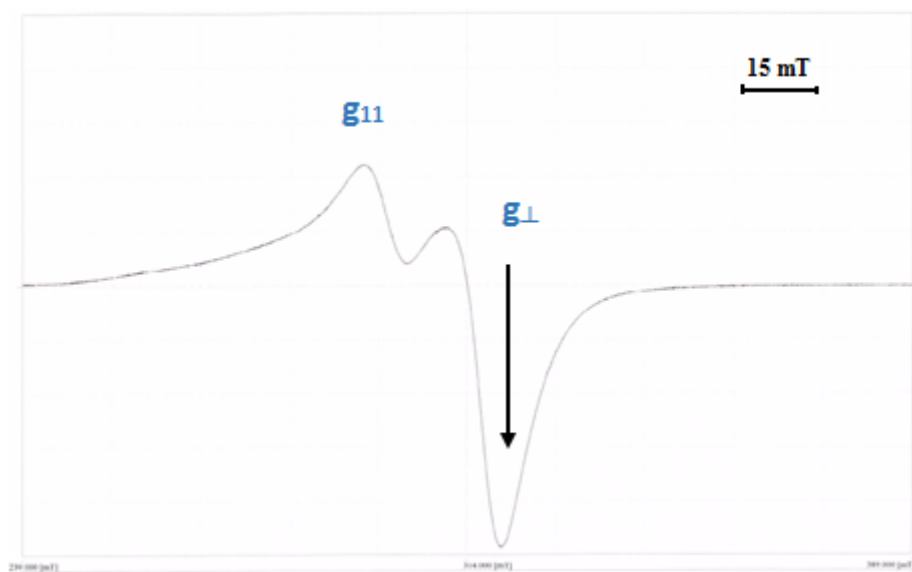
Figure S21. ESR spectrum of [\text{Cu}(\text{MeNap-Pz})_2(\text{NO}_3)]\text{NO}_3 \cdot 2\text{H}_2\text{O} complex.
