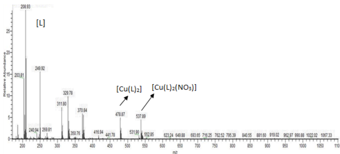
Figure S16. Mass spectrum of [\text{Cu}(\text{NapMe-Pz})_2(\text{NO}_3)_2] \cdot \text{H}_2\text{O} complex.
