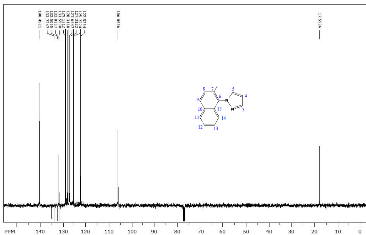
Figure S6. ^{13}\text{C} -NMR (ATP) spectrum of MeNap-Pz ligand recorded in \text{CDCl}_3 and 100.6 MHz.
