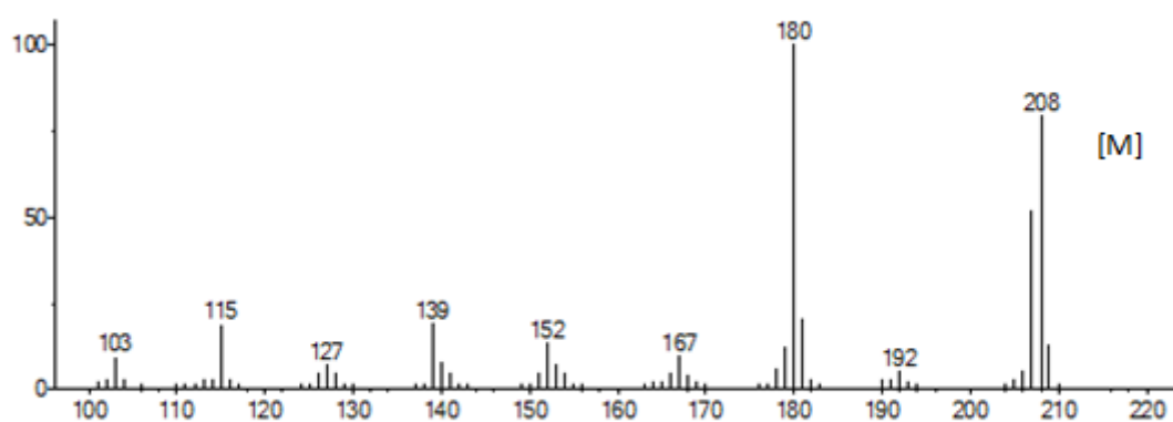
Figure S14. Mass spectrum of MeNap-Pz ligand.
