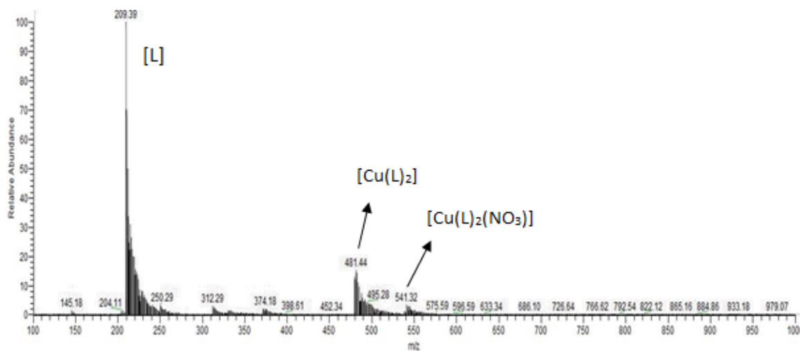
Figure S17. Mass spectrum of [\text{Cu}(\text{MeNap-Pz})_2(\text{NO}_3)]\text{NO}_3 \cdot 2\text{H}_2\text{O} complex.
