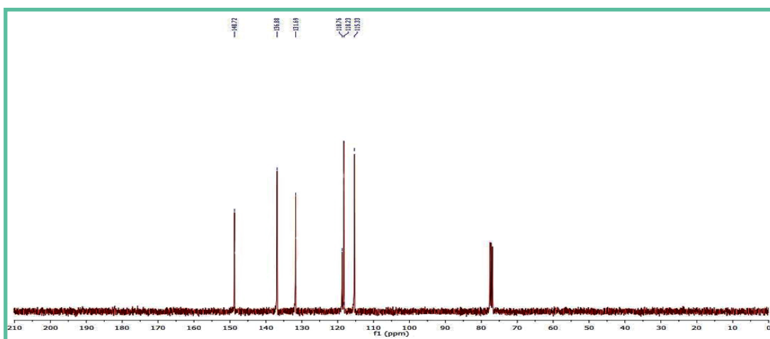
Figure S15. Compound 2 ^{13}\text{C} NMR spectrum.
