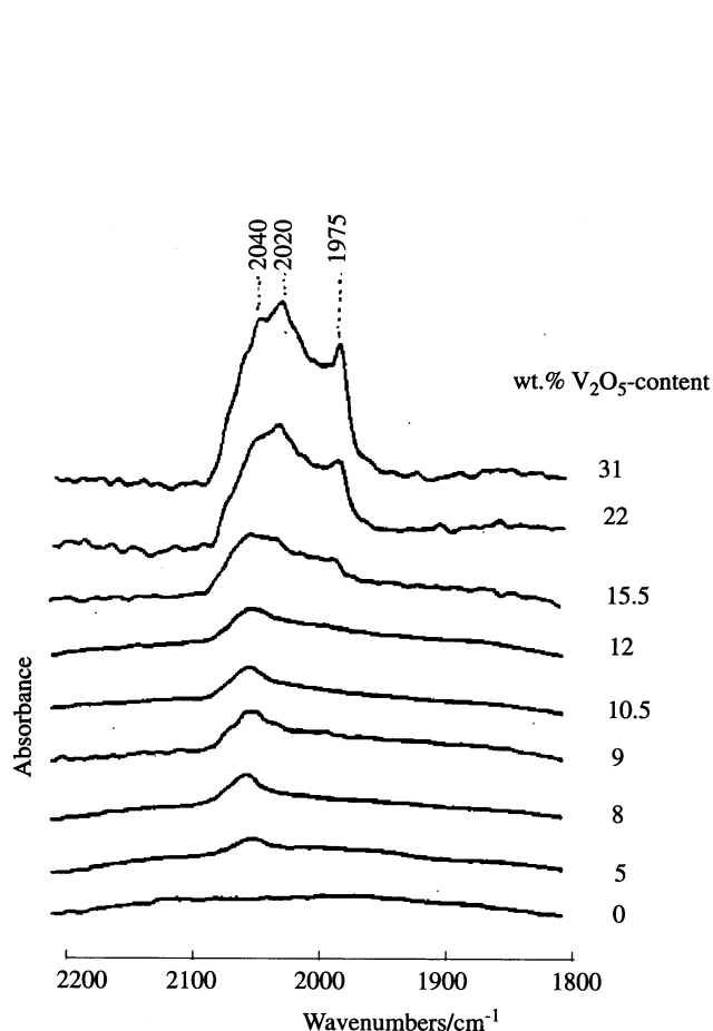
Figure 2. Overtone vibrational bands of V=O of TiO_2(A) and the V_2O_5/TiO_2(A) catalysts
