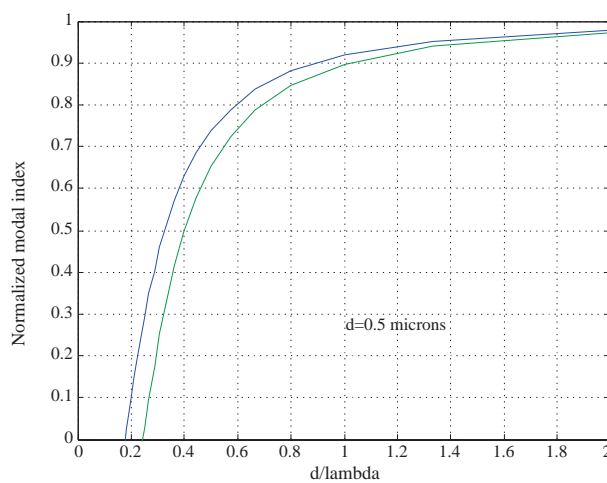
Figure 4. Dispersion characteristics of the first two modes in Guide 3.
