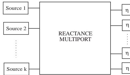
Figure 13. Equivalent circuit of the modified complete radiating electromagnetic structure.
