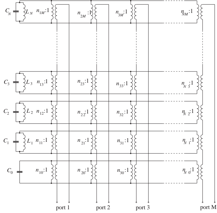
Figure 7. Foster impedance representation of a multiport
