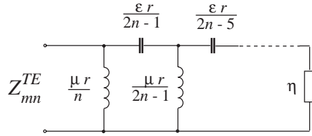
Figure 10. Equivalent circuit of TE_{mn} spherical wave.
