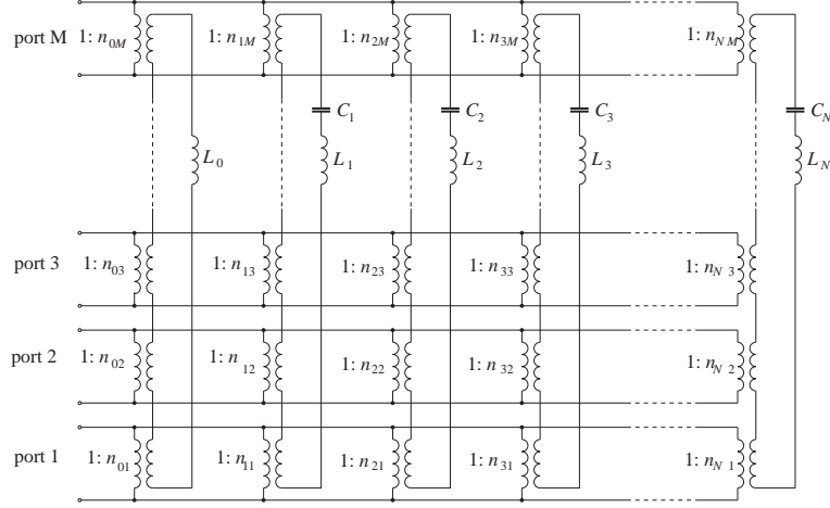
Figure 5. Foster admittance representation of a multiport.
