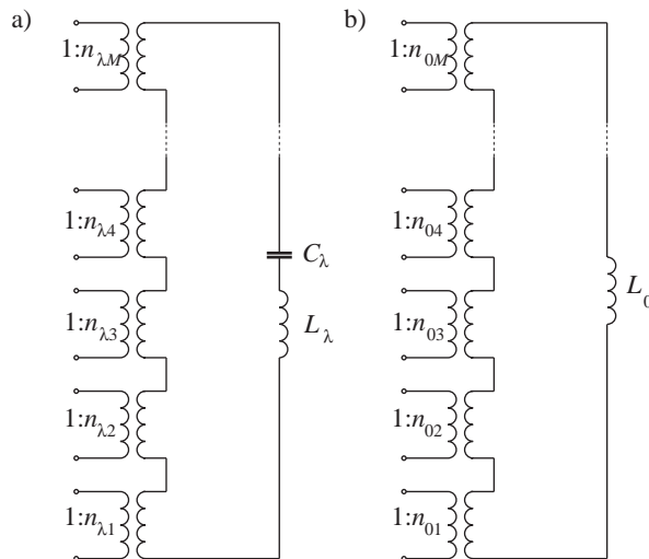
Figure 4. A compact series multiport element representing a pole a) at \omega = \omega_\lambda and b) at \omega = 0 .
