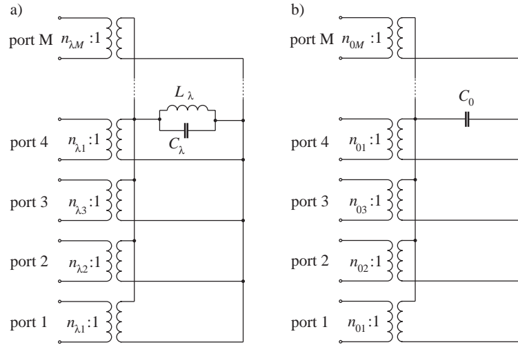
Figure 6. A compact parallel multiport element representing a pole a) at \omega = \omega_\lambda and b) at \omega = 0 .
