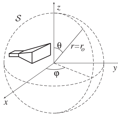
Figure 8. Embedding of an electromagnetic structure into a sphere.
