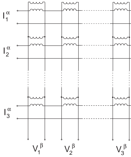
Figure 3. Canonical form of the connection network.
