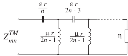
Figure 9. Equivalent circuit of TM_{mn} spherical wave.
