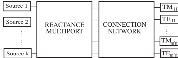
Figure 12. Equivalent circuit of the complete radiating electromagnetic structure.
