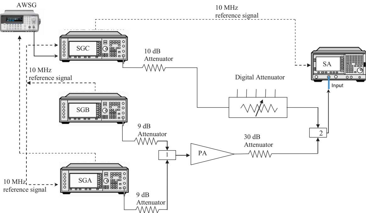
Figure 2. Schematic representation of the measurement setup.
