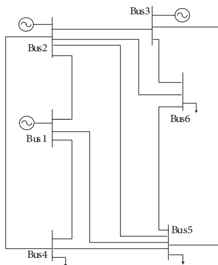
Figure 12. Studied 6-bus power system.
