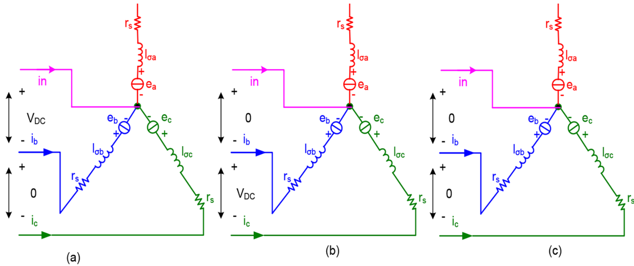
Figure 8. Stator circuits when: (a) V1 is applied; (b) V2 is applied; (c) V0 is applied under phase a open circuit fault.
