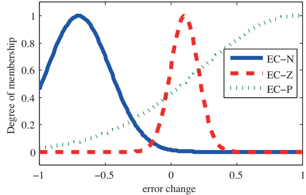
Figure 4. Obtained MFs of input 2 ( e_c ) after optimization by ABC.
