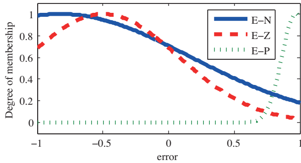
Figure 3. Obtained MFs of input 1 ( e ) after optimization by ABC.
