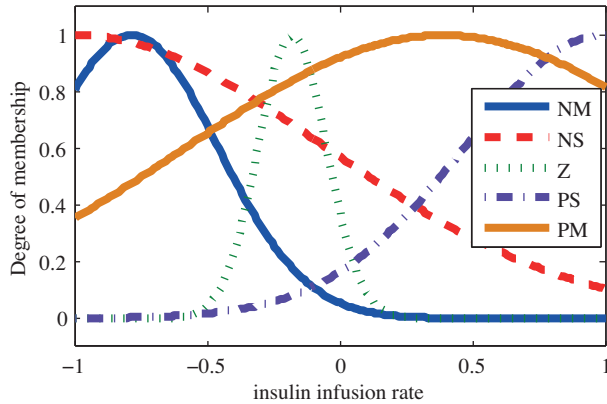
Figure 5. Obtained MFs of output ( u ) after optimization by ABC.
