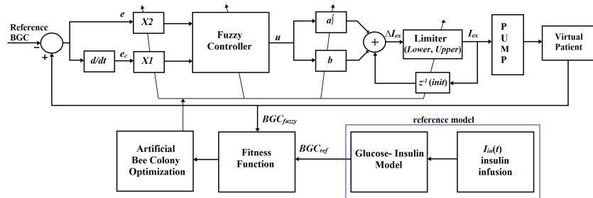
Figure 2. Block diagram of the optimized fuzzy-PID controller.
