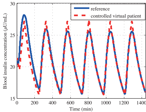
Figure 7. BIC profiles of the reference model and the controlled virtual patient.
