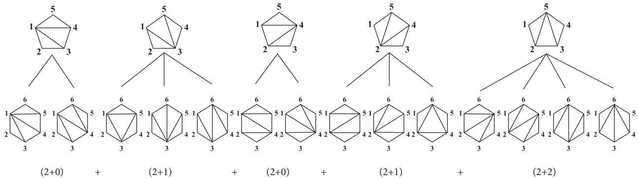
Figure 1. Levels five and six of the tree of triangulations based on decomposition of the Catalan numbers.
