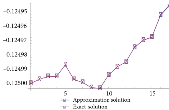
Figure 1. Exact and approximation solution of example 1 for n = 16 , m = 200 , and t = 0.05 .
