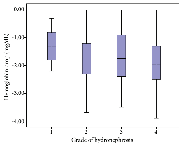
Figure 3. Box-plot graphic between grade of hydronephrosis and bleeding.
