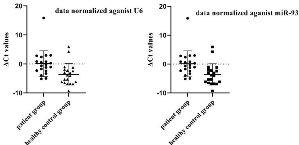
Figure 2a. Distribution of miR-144 \Delta Ct values among the patient and the healthy control groups. When data were normalized against U6, STD values for the healthy control and the patient groups were 2.88 and 3.76, respectively. When data were normalized against miR-93, STD values for the healthy control and the patient groups were 4.45 and 3.73, respectively.
