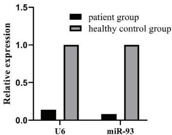
Figure 2b. Changes in mean miR-144 expression levels in serum samples. Data were normalized against U6 (p: 0.017) or miR-93 (p: 0.002) and statistical significance was tested by Manny-Whitney U-test.
