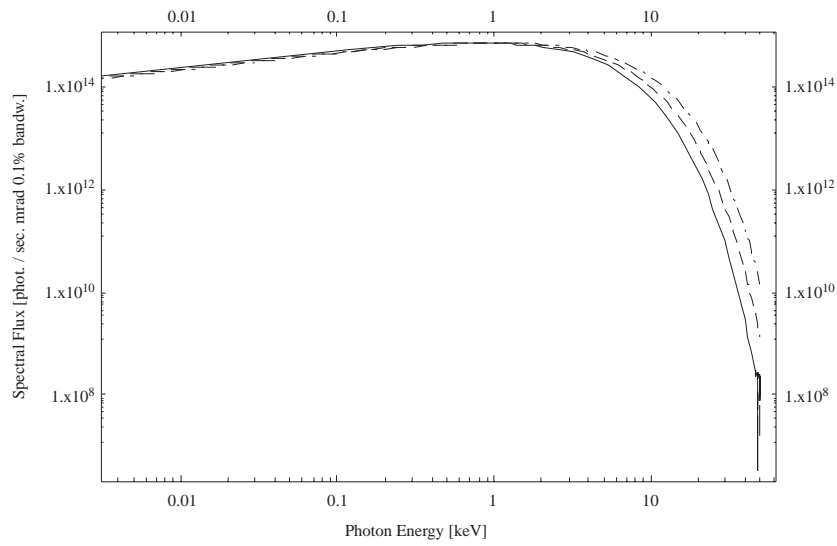
Figure 4. Spectral flux of the SR. Solid line: g=30\text{mm} , Dashed line: g=25\text{ mm} , Dot-dashed line: g=20\text{mm} .
