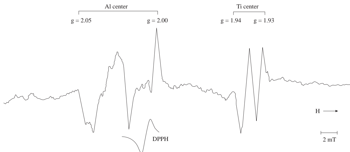
Figure 3. The ESR first derivative spectra of Al and Ti centers in the natural single quartz crystal at 100 K when \mathbf{H} // y ( \mathbf{H} is the applied external magnetic field).
