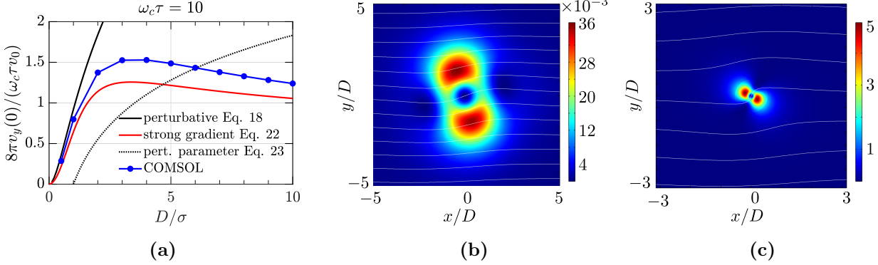
Figure 2. a) Normalized transverse velocity at the center of magnetic region, fixed as origin, plotted against the sharpness of the Gaussian magnetic field distribution with standard deviation \sigma . A strong magnetic field \omega_c \tau = 10 is chosen to highlight the transition from perturbative to strong gradient regimes. The solid black line shows the soft gradient perturbation theory result, which agrees with the numerical solution, as also indicated in Figure 1a. The dotted black line is the perturbation theory parameter A in Equation (5.5). The perturbation theory breaks down when the parameter A \approx 0.5 . The solid red curve is from the strong gradient solution Equation (5.4), which shows the logarithmic suppression at the origin. The COMSOL Multiphysics [42] simulations, shown by the blue dots, agree with the strong gradient calculation up to logarithmic accuracy. b-c) Distribution of viscous power density in real space, normalized to the uniform ohmic dissipation (nev_0)^2 \rho_\tau \approx 0.05 \text{ W/m}^2 . The simulation is performed on COMSOL. The white curves are the streamlines. The magnetic field is chosen to be large ( \omega_c \tau = 10 ) for better visibility of streamline deformation. The viscous dissipation is due to a Gaussian magnetic field distribution with standard deviation \sigma . The perturbative limit with soft gradient \sigma = D is shown in (b) and the strong field, strong gradient \sigma = D/10 is realized in (c). Note that the power dissipation is suppressed at the origin, which is a consequence of the Gaussian magnetic field distribution.
