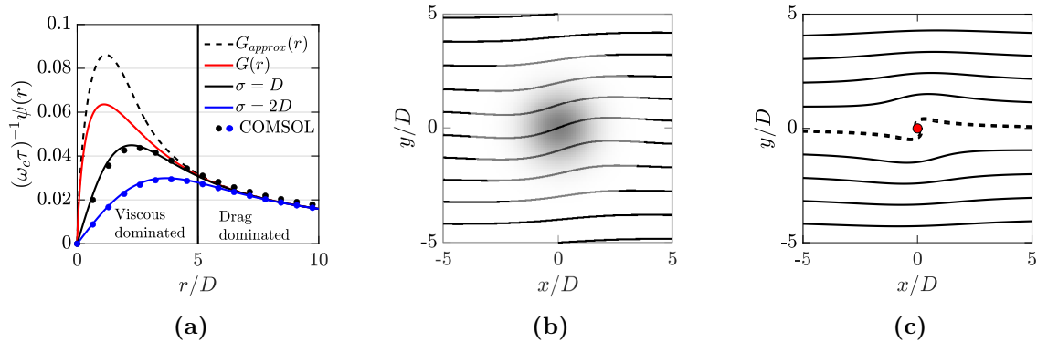
Figure 1. The electrons follow curves of constant streamfunction \Psi , called the streamlines. In the Stokes problem, we assume a uniform flow of electrons in the x -direction is incident on a localized magnetic field region. a) The radial part of the normalized correction to the stream function in the weak field intensity and soft gradient regime. The total streamfunction is \Psi = -v_0 y + v_0 D \psi(r) \cos(\varphi) . The out-of-plane magnetic field \mathbf{B} = \hat{z} B b(r) is assumed to be radially symmetric with a Gaussian profile b(r, \sigma) centered around the origin with a standard deviation \sigma . The solid blue and black curves are the analytic solutions (see Equation (4.12)) for, \sigma = D, 2D , respectively. The filled circles are data points obtained by simulating the system on COMSOL Multiphysics software [42] with weak field parameters. Notice that the blue circles have a closer agreement with theory, since the analytic solution is obtained in the weak gradient limit. In the limit \sigma \rightarrow 0 , the profile becomes a delta function, hence we recover the radial part of the Green's function in Equation (4.11), shown by solid red curve. The flow is viscous dominated close to the origin and drag dominated further away. The transition occurs around r = 5D . The Green's function can be piecewise constructed in these asymptotic regions, respectively, as G_<, G_> in Equation (4.9), shown by the dashed black curve b) The streamlines of an electric current incident on a magnetic field region with soft Gaussian profile. The current in the x -direction is deflected by the out-of-plane magnetic field concentrated in the dark region. c) A magnetic impurity creates a sharply changing magnetic field profile and induces large Lorentz force gradients. Hence, the perturbative solution no longer holds. Instead, the current near the impurity is logarithmically suppressed, therefore the streamline passing through the origin (dashed lined) does not carry current. Here, the small radius of the impurity r_0 = 0.2D serves as the ultraviolet (UV) logarithmic cut-off. In (b) and (c) the magnetic field is exaggerated to make the streamline deformation more prominently visible.
