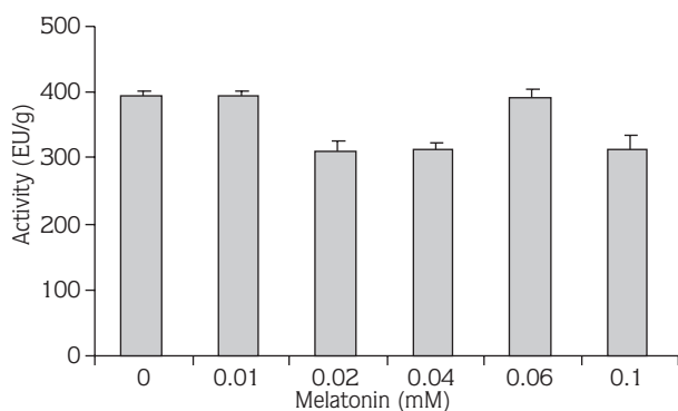
Figure 2. In vitro changes in activity (EU/g) of erythrocyte CA enzyme from O. mykiss in presence of 5 different melatonin hormone concentrations. (0.06 mM is regarded as a pharmacological dose or maximum dose and 0.1 mM as an overdose). Values are expressed as mean \pm SD ( n = 3 ).
