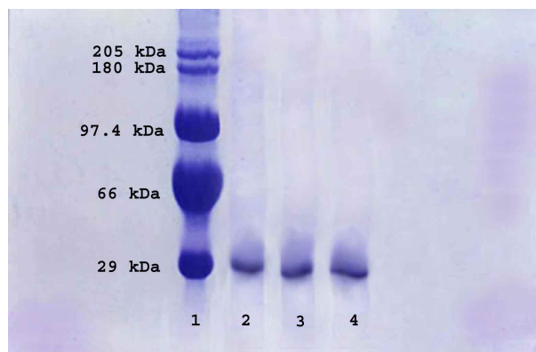
Figure 1. SDS-polyacrylamide gel electrophoresis of CA purified by affinity gel. [(Lane 1: Standard proteins; (Rabbit muscle myosin 205,000 Da, \alpha_2 -Macroglobulin 180,000 Da, rabbit phosphorylase B 97,400 Da, bovine serum albumin 66,000 Da and bovine carbonic anhydrase 29,000 Da) Lane 2: O. mykiss erythrocyte CA; Lane 3: O. mykiss gill CA; Lane 4: O. mykiss lens CA)].
